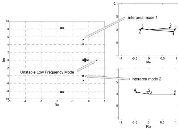
Fig. 2. Uncontrolled system modes of oscillation (without AVR or PSSs).
