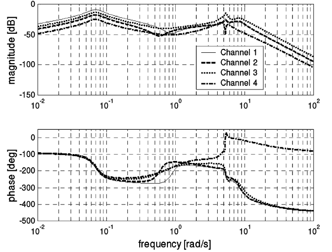
Fig. 9. Bode plots of transfer functions between voltage reference and speed.
