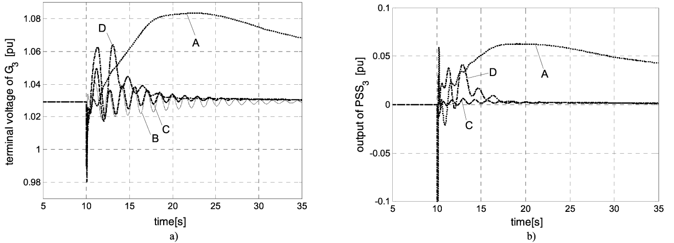
Fig. 6. Response of generator G_3 to 100 ms fault in the vicinity of node 5. (a) Terminal voltage response of generator G_3 for all four AVR/PSS designs. (b) PSS output of generator G_3 for AVR/PSS designs A, C, and D.
