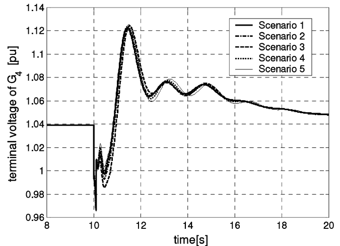
Fig. 12. Response of generator G_4 to 100-ms fault for all five scenarios.
