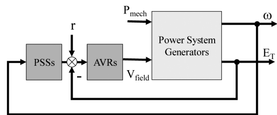
Fig. 4. AVR/PSS configuration.
