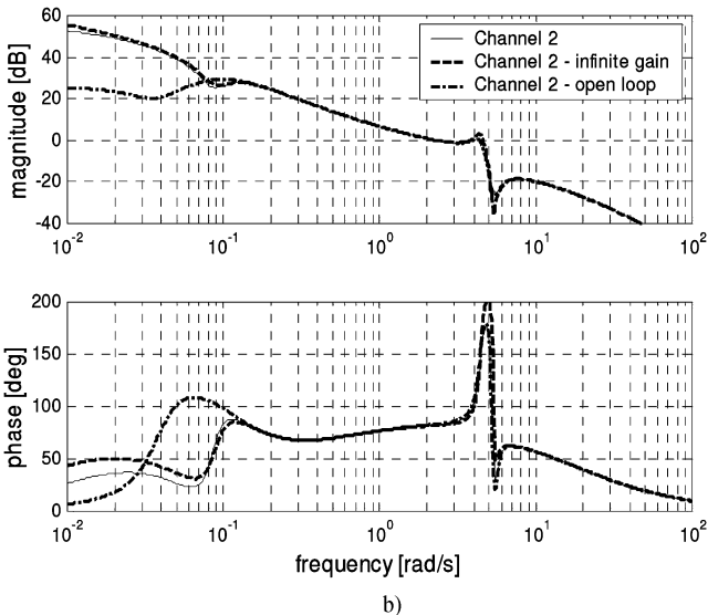
Fig. 11. AVR channels for Design D. (a) Channel 1. (b) Channel 2.
