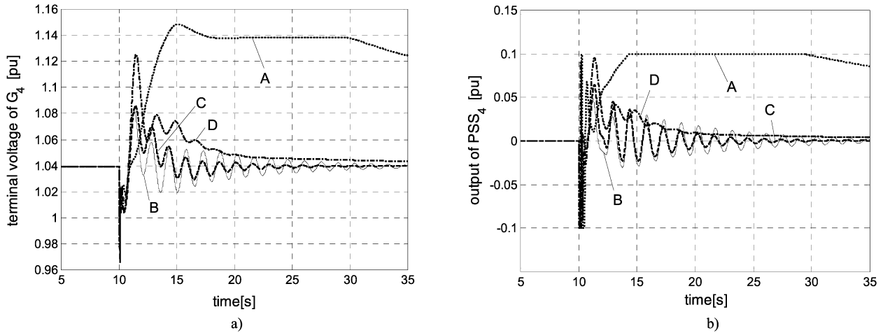
Fig. 7. Response of generator G_4 to 100 ms fault in the vicinity of node 5. (a) Terminal voltage response of generator G_4 for all four AVR/PSS designs. (b) PSS output of generator G_4 for all four AVR/PSS designs.
