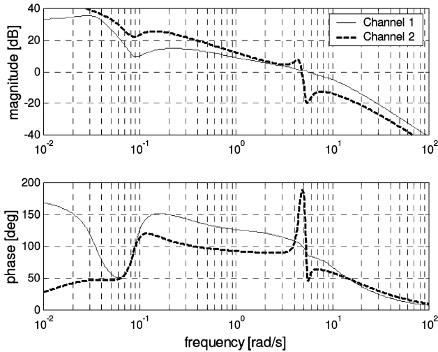
Fig. 10. AVR channels for design B.
