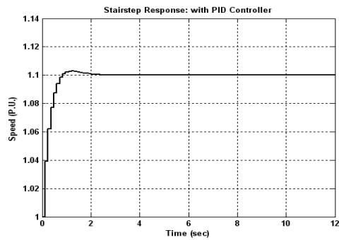
Fig. 26: Stair-step stable response with PID controller
