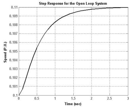
Fig. 2: The Open-loop step response of the motor system using T. F. or state-space; with initial speed=0.1 p.u. at steady state
