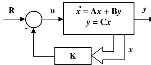
Fig. 18: The schematic for a full-state feedback system
